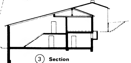
3 Section
